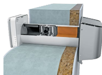
Unit installation example with the hood for thin walls AH-S grey 160 / AH-S chrome 160
