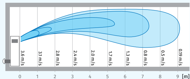
Fresh air flow distance for CIVIC EC LB 500 V.2
