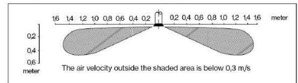
Distribution pattern at 110m³/s at 4.8 mm and 30 dB(A)
