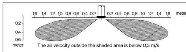
Distribution pattern at 70m 3 /h at 7 mm and 30 dB(A)
