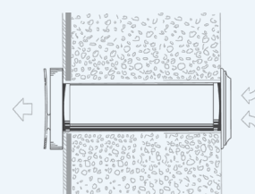
Wall installation
