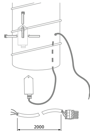
In the exhaust air duct upstream of the heat exchanger (only for KOMFORT EC S(B) 160(-E))
