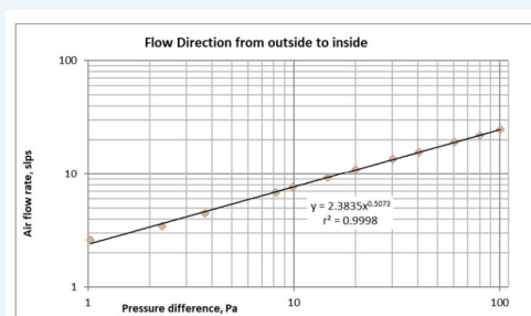
Figure 5 Measured air flow and pressure data for air flow from outside to inside corrected to STP.
